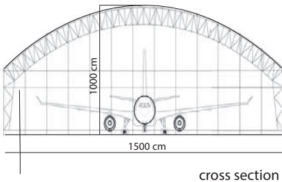
cross section
